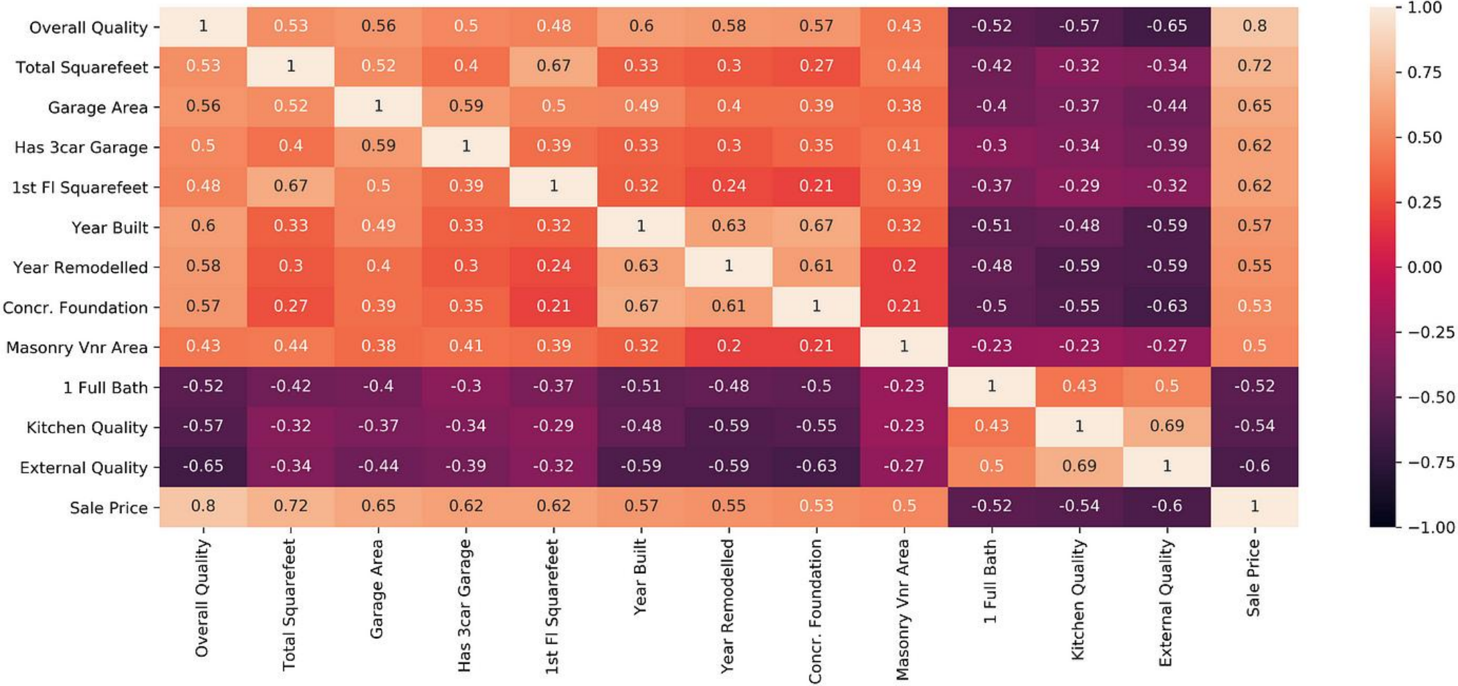
Correlation Heatmap
